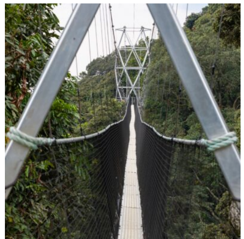
Canopy Walkway
